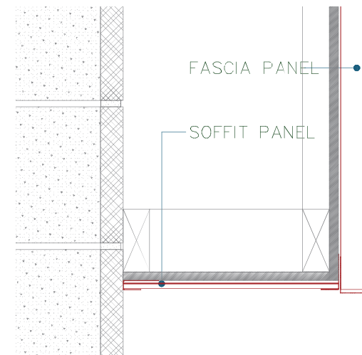
TYPICAL SYSTEM INSTALLATION
